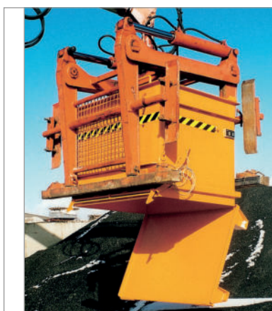
BC with brick clamp operated drop away base
