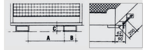
Fork sleeve inside dimensions in mm
