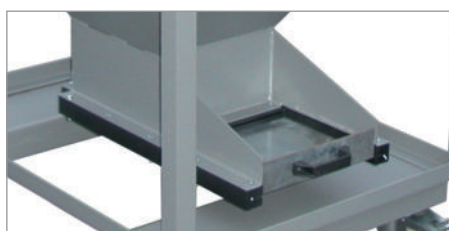
Sliding gate with a special seal on the hopper floor (SR-D, SG-D, SRE-D)
