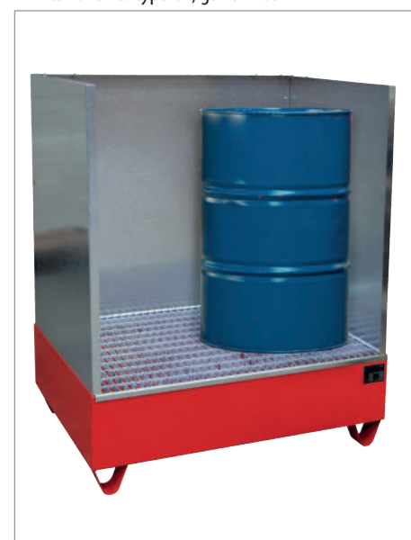
2018/SW (with splash protection walls)
